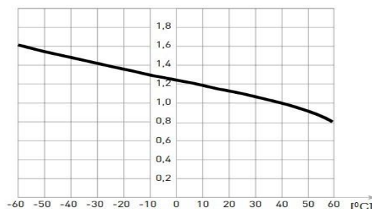
Fig. 6. The dependence of the rated current of automatic ambient temperature switch
