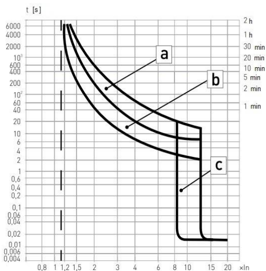
a - release response from the “cold” state at overload currents; b - release response from the “warm” state at overload currents; c - release response at short circuit currents.
