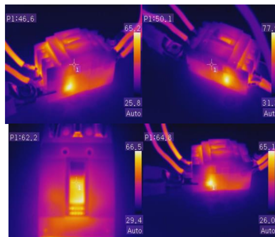
Fig. 7. The figure shows the thermal imaging of the circuit breaker heating, with a bimetallic plate, when operating in nominal mode (the maximum heating temperature is indicated in the upper left corner)
