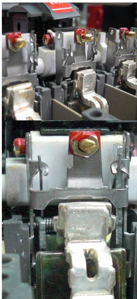
Fig. 2. General image of the CB releasers
