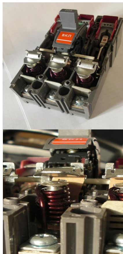
Fig. 3. Releaser with electro-hydraulic retardation
